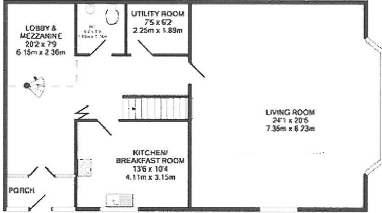
GROUND FLOOR APPROX. FLOOR AREA 1037 SQ. FT. (96.4 SQ. M.)
